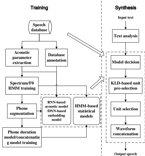
Figure 1: Flowchart of the Our unit selection system.
